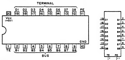
SN75160AN (TI) SN75160AN-R (TI) SN75160N (TI) OCTAL GENERAL-PURPOSE INTERFACE BUS TRANSCEIVERS — TOP VIEW —
